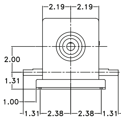
STANDARD MOUNT
